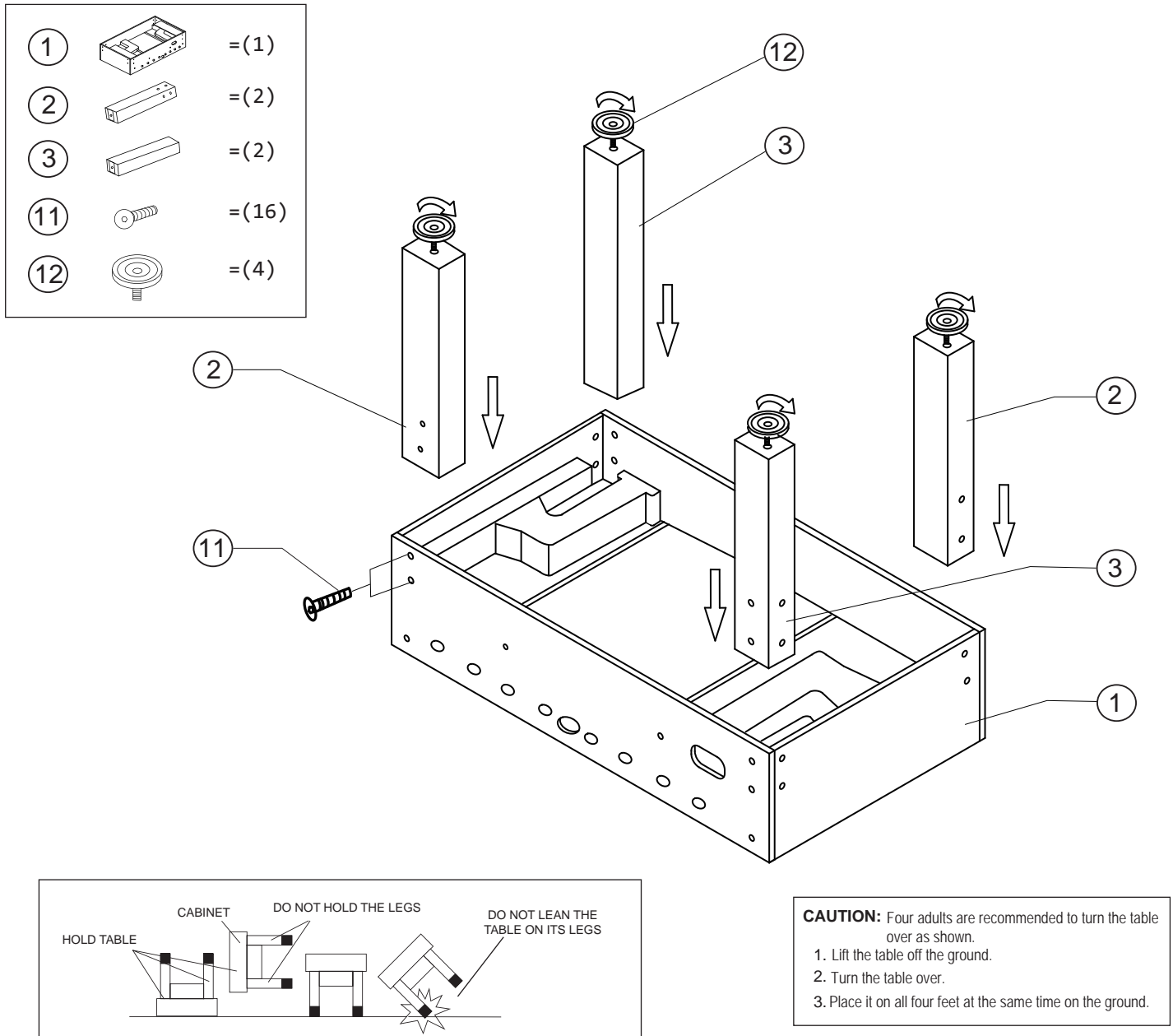
FIG. 1: LEG ASSEMBLY
